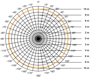
Surface-mounted installation, square For further designs, see page 54
