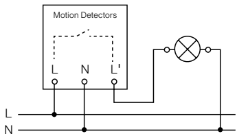
Further circuit diagrams starting on page 284
