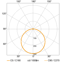
Light distribution curve for RS PRO LED S2, PC
