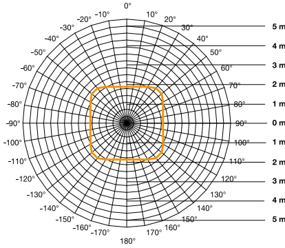
Detection zone for IR Quattro SLIM XS installed at a height of 2.80 m orange = tangential, radial, presence
