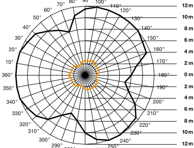
Detection zone IS300 mounted at a height of 2.5 m black = tangential walking direction orange = radial walking direction
