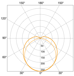
Light distribution curve for L 665 LED
