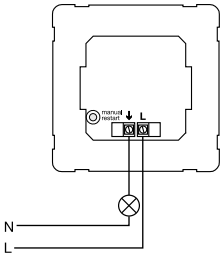
Also suitable for parallel operating mode. Further circuit diagrams starting on page 286
