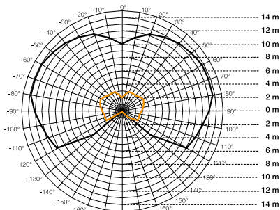
Detection zone for XLED PRO Wide mounted at a height of 2.8 m black = tangential walking direction orange = radial walking direction
