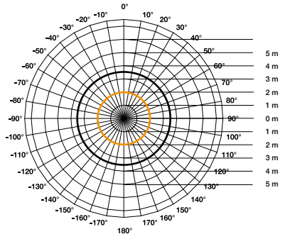
Detection zone IS2360ECO mounted at a height of 2.8 m black = tangential walking direction orange = radial walking direction
