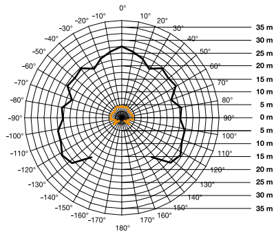
Detection zone for sensIQ S mounted at a height of 2.5 m black = tangential walking direction orange = radial walking direction
