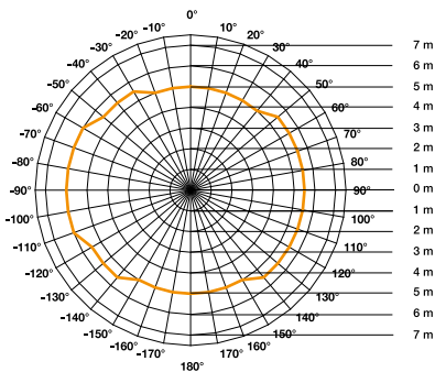
Detection zone for RS PRO LED S1 IP65 mounted at a height of 2.8 m orange = radial walking direction
