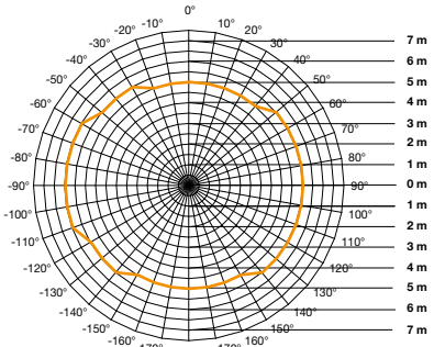
RS 10 L detection zone Mounting height 2.8 m orange = radial walking direction
