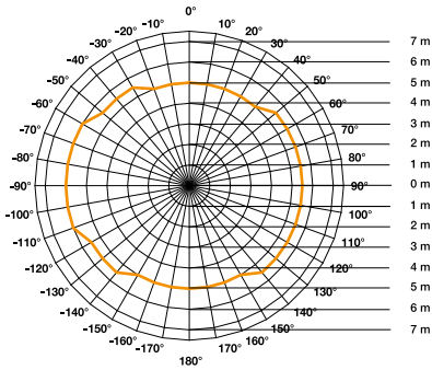
Detection zone for RS PRO LED S1 mounted at a height of 2.8 m orange = radial walking direction
