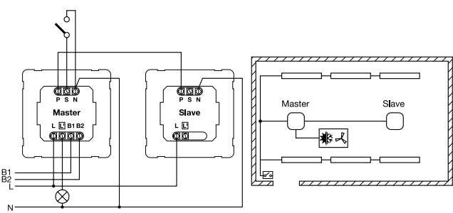
Master-slave
