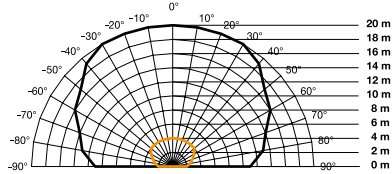
Detection zone for IS 2180-5 20 m lens black = tangential walking direction orange = radial walking direction
