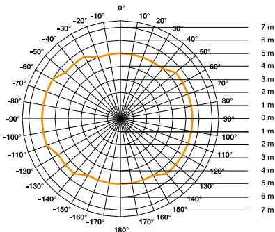
Detection zone for RS PRO LED S2 IP65 mounted at a height of 2.8 m orange = radial walking direction
