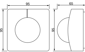
Surface-mounted installation, square For further designs, see page xxx
