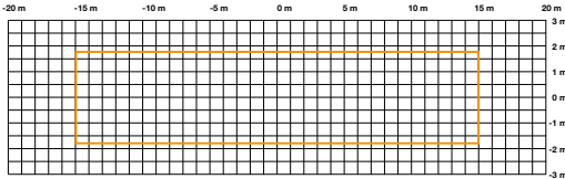
Detection zone for IS345 MX Highbay mounted at a height of 12.5 m orange = radial walking direction
