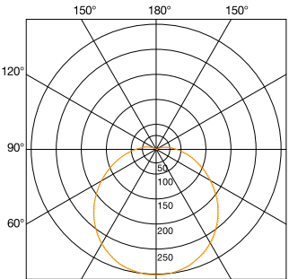
— C0 / C180 cd/1000lm — C90 / C270 RS PRO LED R1 light distribution curve
