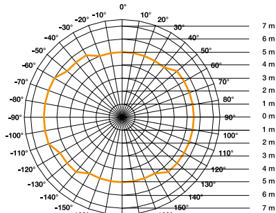
Detection zone for RS PRO DL LED 20W mounted at a height of 2.8 m orange = radial walking direction
