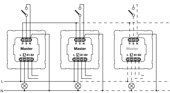
Master/master COM1/COM2
