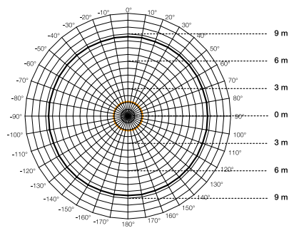
Detection zone for L 691 LED mounted at a height of 2.8 m black = tangential walking direction orange = radial walking direction
