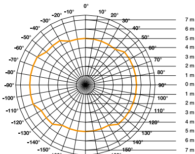
Detection zone for RS PRO LED B1 mounted at a height of 2.8 m orange = radial walking direction
