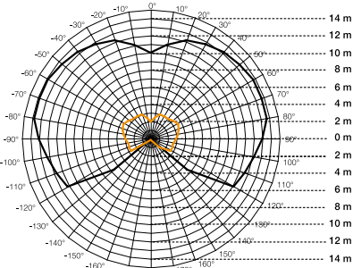
Detection zone for L 400 S mounted at a height of 2.8 m black = tangential walking direction orange = radial walking direction
