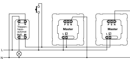
2 detectors linked with an external stairwell lighting timer Old building / building modernisation
