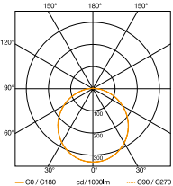
Light distribution curve for RS PRO LED S1 PC
