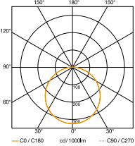
Light distribution curve for RS PRO LED S1 glass
