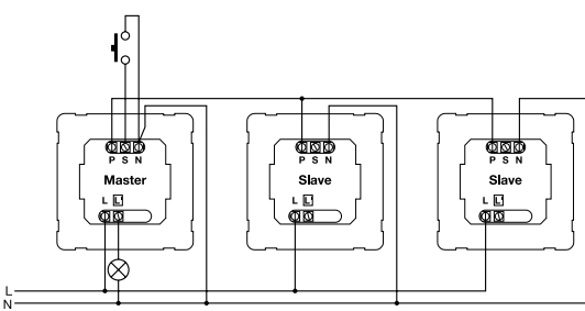
Detector connected to stairwell lighting timer
