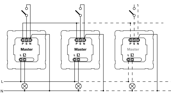
Master/master COM1
