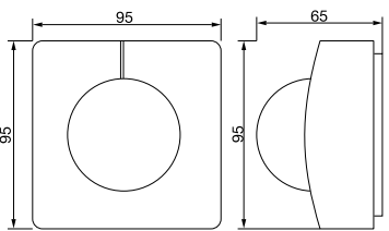
Surface-mounted installation, square For further designs, see page 54
