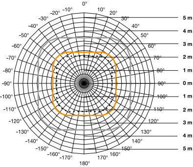
IR Quattro detection zone Installation height 2.80 m grey = tangential orange = radial black = presence
