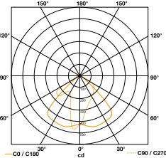
Light distribution curve for XLED PRO Square XL
