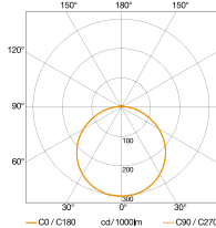
Light distribution curve for RS PRO LED S2, PMMA
