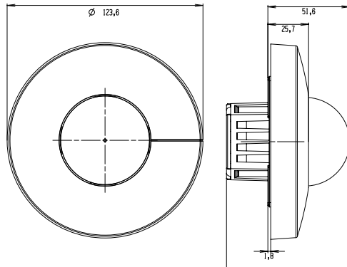
Concealed installation, round
