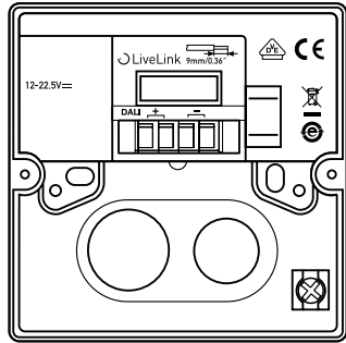
Surface-mounted installation
