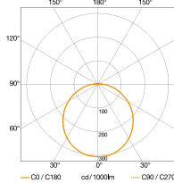
Light distribution curve for RS PRO LED S2, glass
