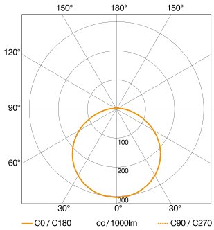
Light distribution curve for RS PRO LED S2 IP65
