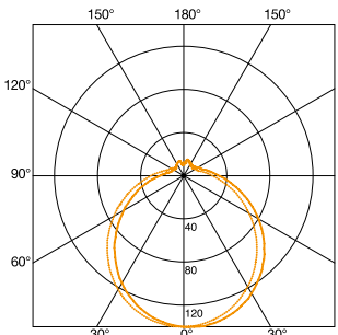
Light distribution curve for RS 10 L
