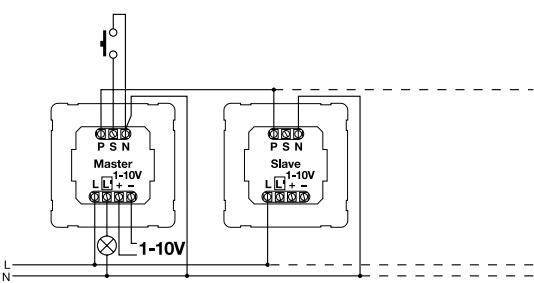
DIM detector with slave
