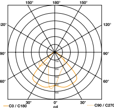
Light distribution curve for XLED PRO Square
