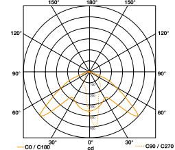
Light distribution curve for XLED PRO Wide
