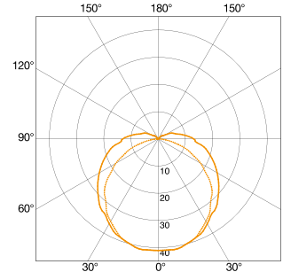
Light distribution curve for L 666 LED
