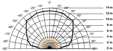
Detection zone for IS2180-2 12 m lens black = tangential walking direction orange = radial walking direction
